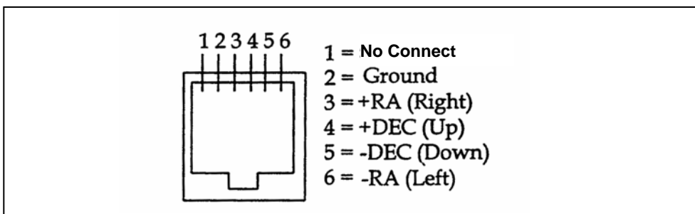
Figure 8-7 – Pin out diagram for Autoguider port.
